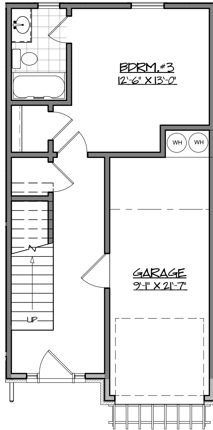
1ST FLOOR
