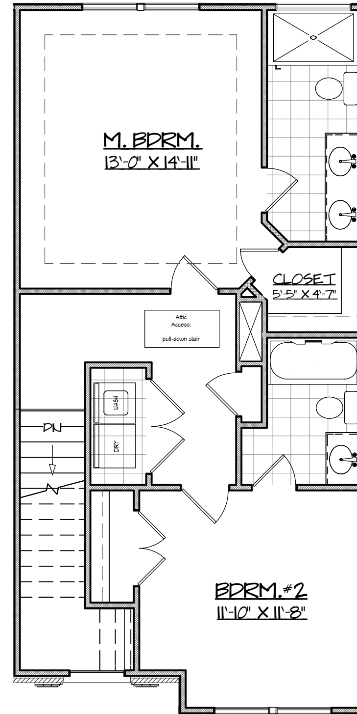
3RD FLOOR
